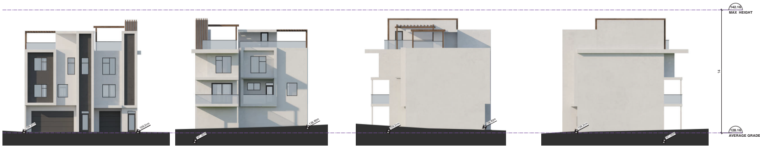
2 Building 7 A005 Scale: 3/32"=1"
